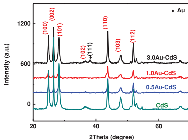
Figure 5f. XRD patterns of the prepared CdS SNPs and CdS SNPs-Au NPs hybrids with different weight addition ratios of Au NPs.
